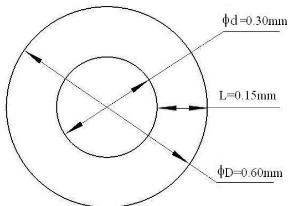
Figure 2. Mechanical dimensions of ATTB30B
