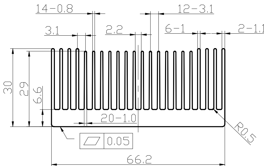
Figure 5. Mechanical Dimensions of Heat Sink ATHS-1/2/105/66/30A
