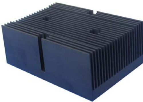
Figure 2. The Physical Photo of ATHS-1/2/105/66/30H4
